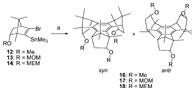
Scheme 8. Synthesis of cyclotrimers 16 , 17 , 18 . Reagents and conditions: a) \text{CuTC} , NMP, 0 °C to room temperature [ syn - 16 (78%), syn - 17 (72%), syn - 18 (77%)].
