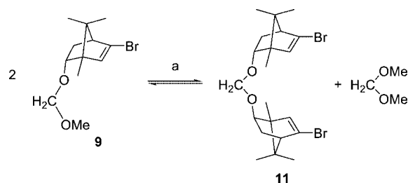
Scheme 5. Equilibrium between acetals 9 and 11 . Reagents and conditions: a) traces of silica gel, room temperature (variable amounts).
