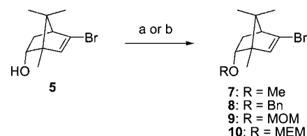
Scheme 4. Protection of the bromobornenol 5 . Reagents and conditions: a) i) \text{NaH} , \text{Et}_2\text{O} , 0^\circ\text{C} ; ii) \text{MeI} or \text{BnBr} (80 or 74%); b) \text{MOMCl} or \text{MEMCl} , i\text{Pr}_2\text{NEt} , \text{CH}_2\text{Cl}_2 , room temperature (95 or 92%).
