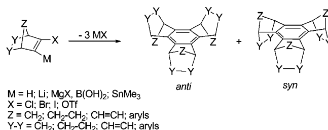
Scheme 1. Synthesis of benzocyclotrimers using the cyclotrimerization reaction leads to formation of the syn and anti isomers. The most typical system involves the presence of a double bond with vicinal halogen and metal substituents.
