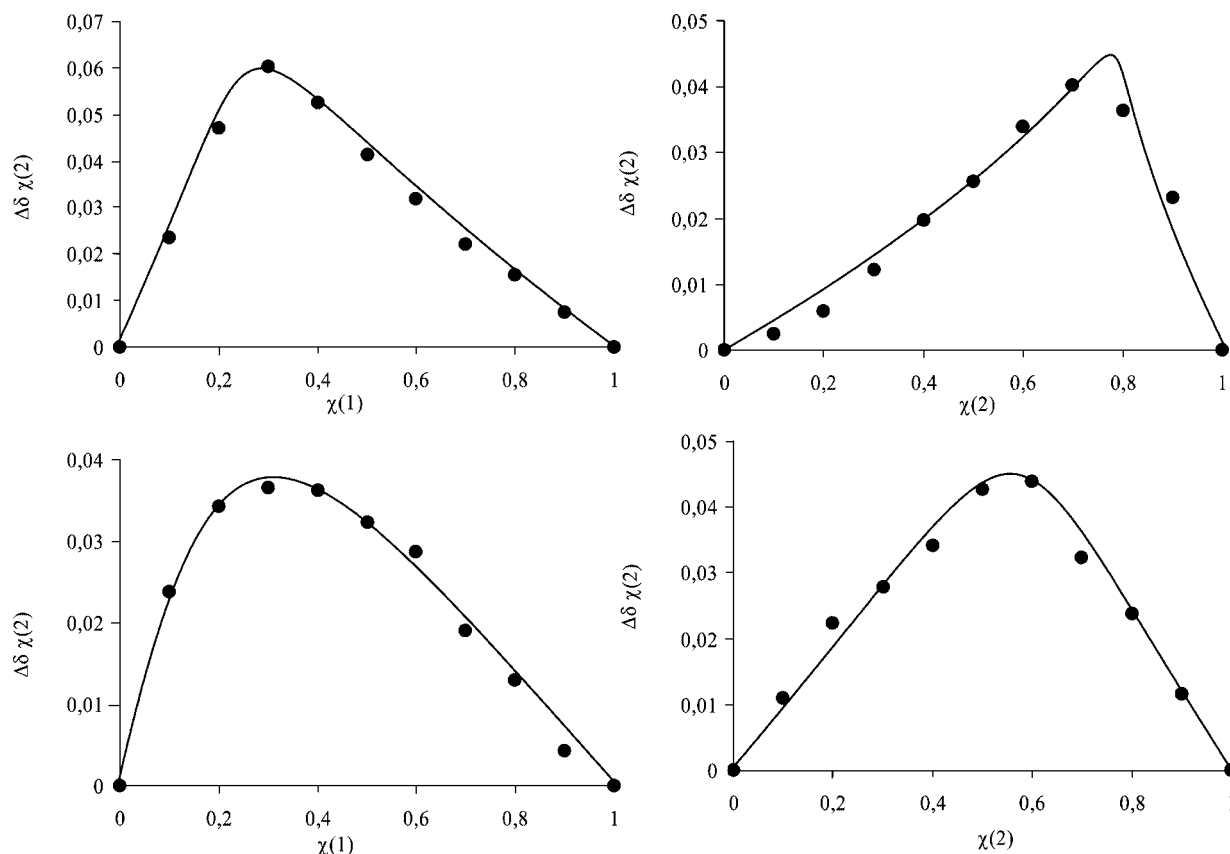
Figure 2. ^1\text{H} NMR Job plots for the binary mixtures syn-1 and (+)- 19 and (–)- 19 .
