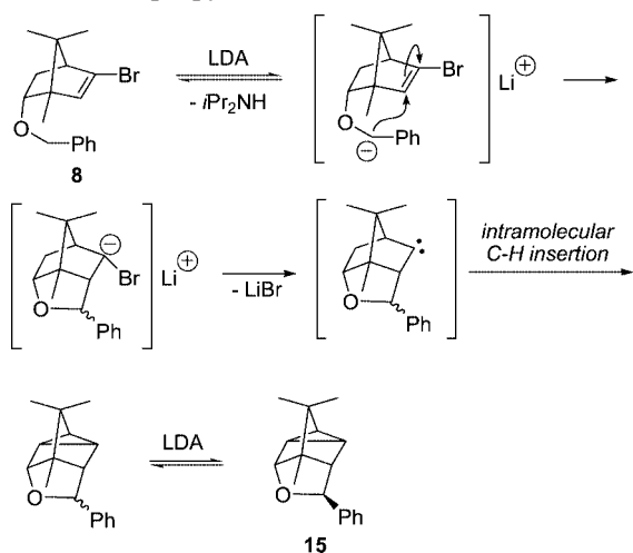
Scheme 7. Proposed mechanism of formation of 15 .
