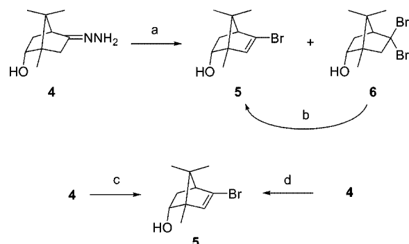
Scheme 3. Synthesis of the bromobornenol 5 . Reagents and conditions: a) \text{PyHBr}_3 , \text{Py} , \text{Et}_2\text{O} , room temperature, (2:1 ratio); b) t BuOK, DMSO, 0^\circ\text{C} (58%); c) NBS, \text{Py} , 0^\circ\text{C} (62%); d) \text{Br}_2 , t BuOK, \text{Et}_2\text{O} , room temperature (74%).
