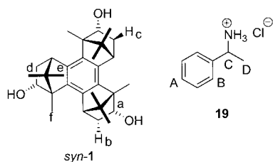
Figure 3. Proton labelling scheme for the titrations of Table 2.
