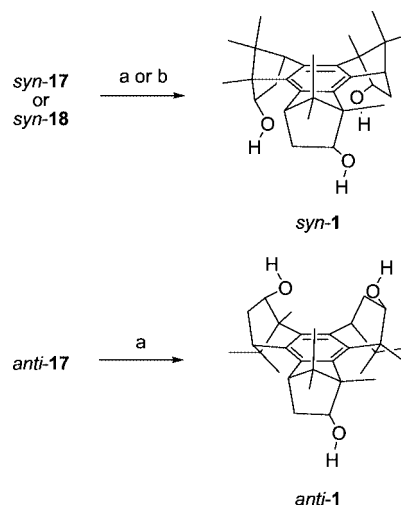
Scheme 9. Deprotection of cyclotrimers 17 and 18 . Reagents and conditions: a) concd. HCl, MeOH, room temperature (quant.); b) acid resin, MeOH, 70 °C (quant.).
