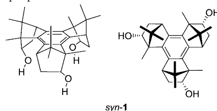
Figure 1. syn -Benzotriborneol syn - 1 presents three hydroxy groups in a rigid conformation describing a hydrophilic cavity.
