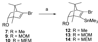
Scheme 6. Stannylation of protected bornenols 7 , 9 , 10 . Reagents and conditions: a) i) LDA, THF, room temperature; ii) \text{Me}_3\text{SnCl} (83, 86, 93%).
